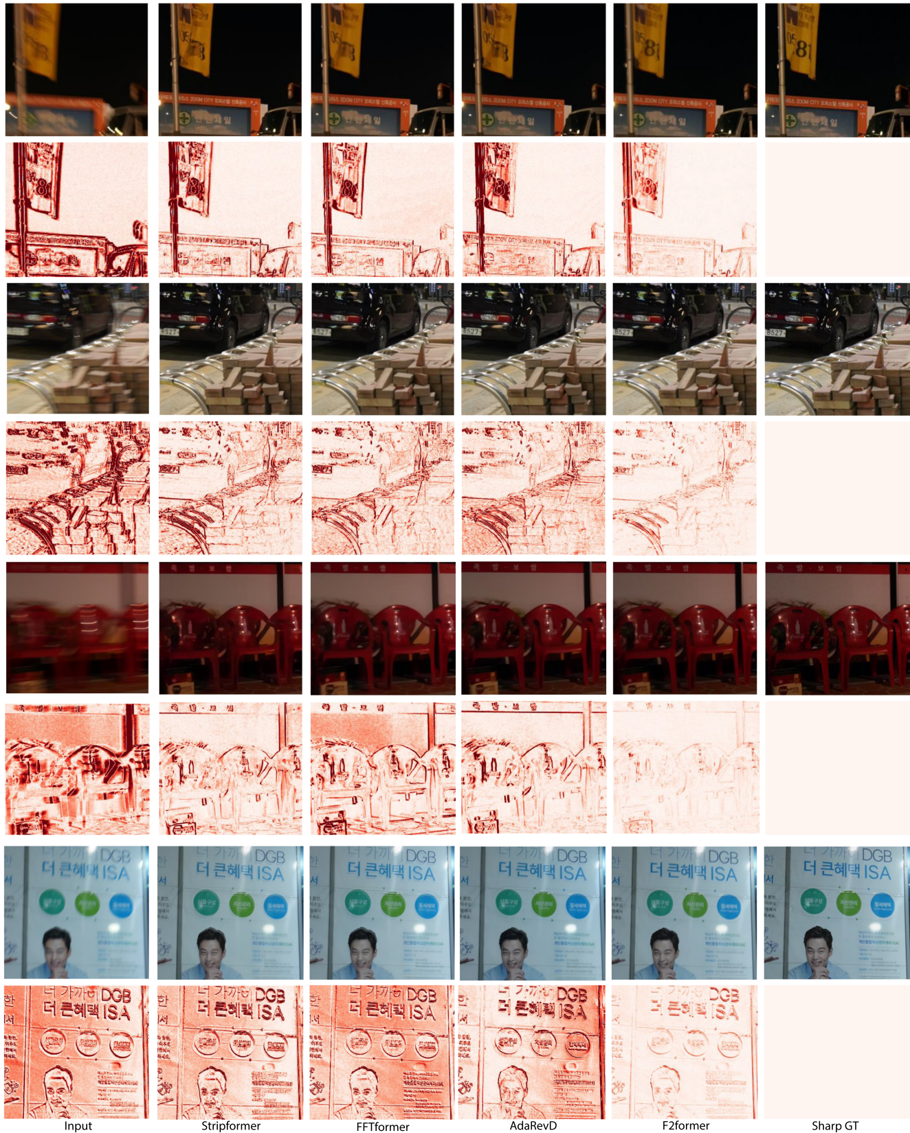
Figure 11: Examples on the RealBlur-J test dataset. The odd rows show blur image, predicted images of different methods, and GT sharp image. The even rows show the corresponding residual of the blur image / predicted sharp images and GT sharp image. Better visualized at 200%.
