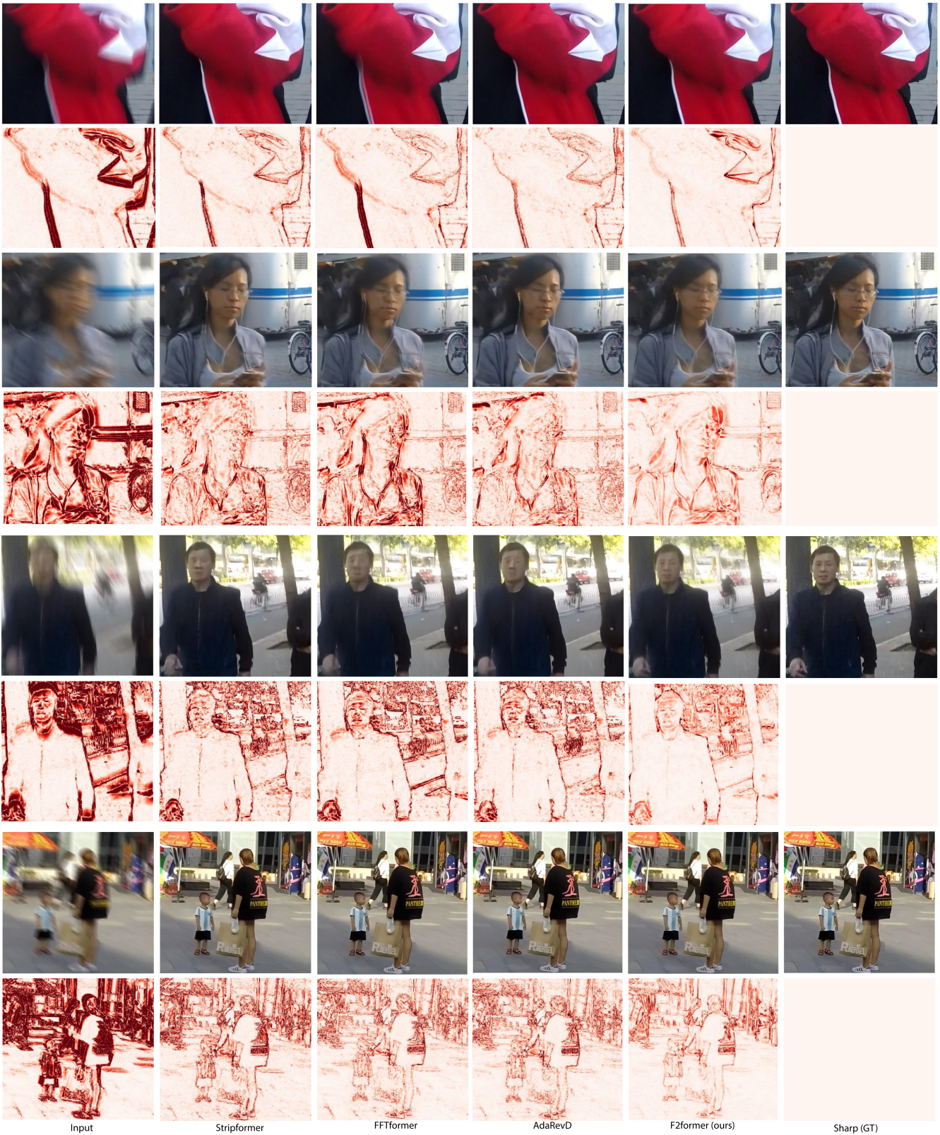
Figure 12: Examples on the HIDE test dataset. The odd rows show blur image, predicted images of different methods, and GT sharp image. The even rows show the corresponding residual of the blur image / predicted sharp images and GT sharp image. Better visualized at 200%.
